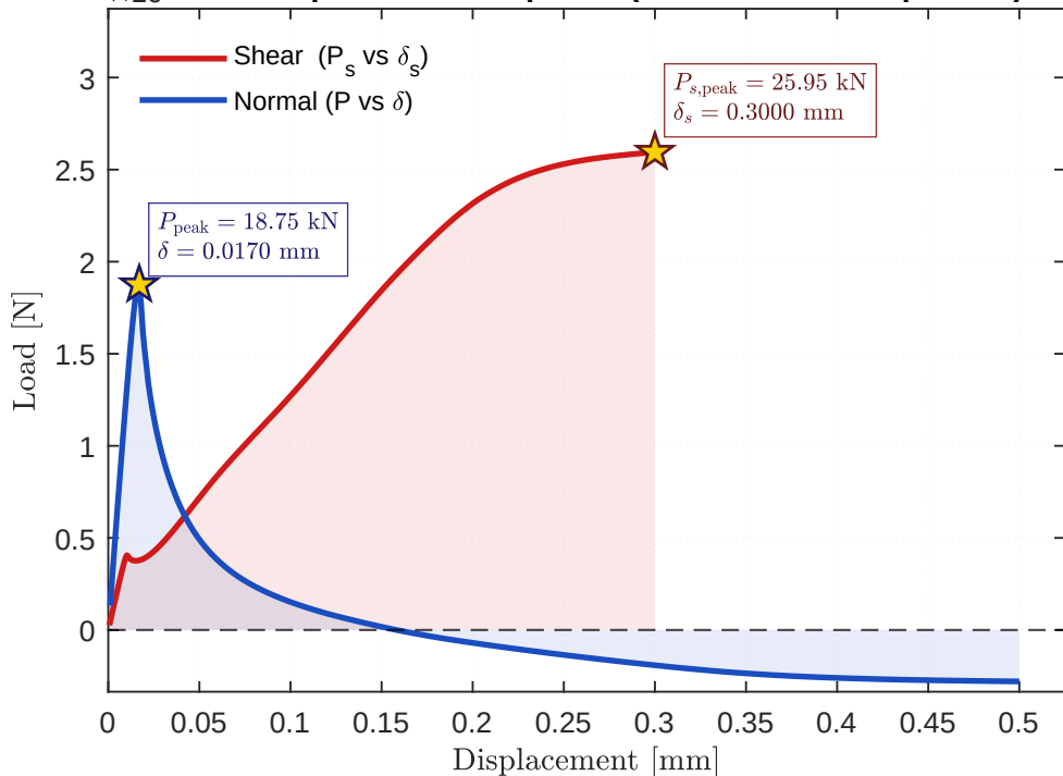
L4 Load -- displacement response (Nooru-Mohamed path 4c)
